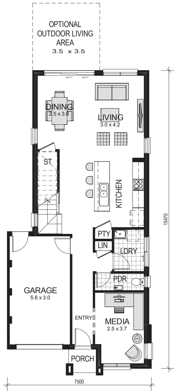
GROUND FLOOR
